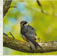
Falco subbuteo <SPRING> <SUMMER> <FALL>
