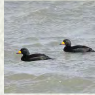
Melanitta nigra <SPRING> <FALL> <WINTER>
